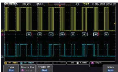
Decode by Analog Channel
