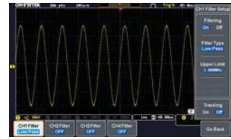
Filtered Waveform, Noise Removed
