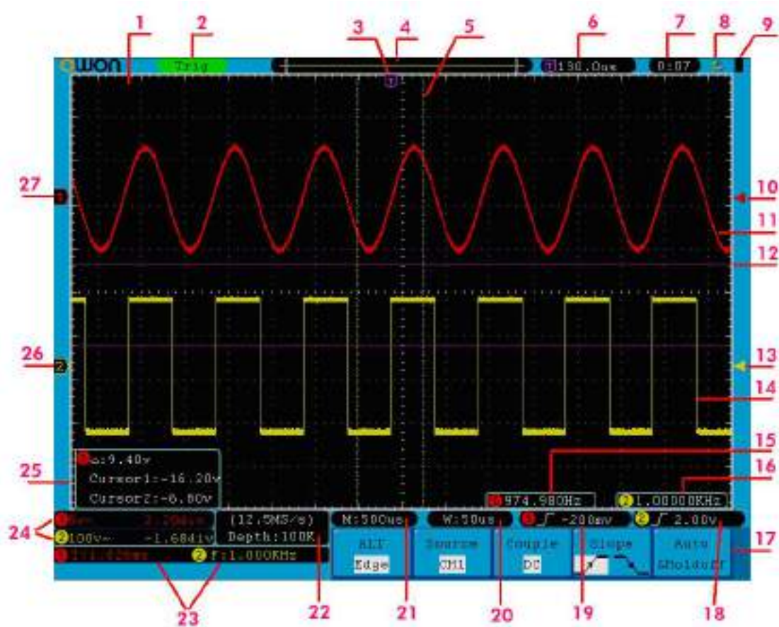
Fig. 4-6 Illustrative Drawing of Display Interfaces
