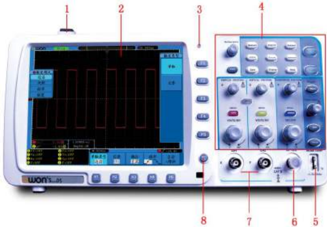
Fig. 4-1 Front panel
