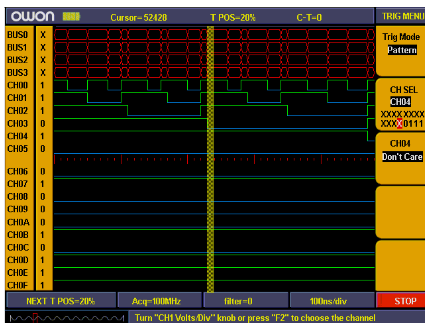
Fig.5-59: Pattern trigger
