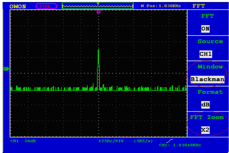
Fig.5-9. Blackman window
