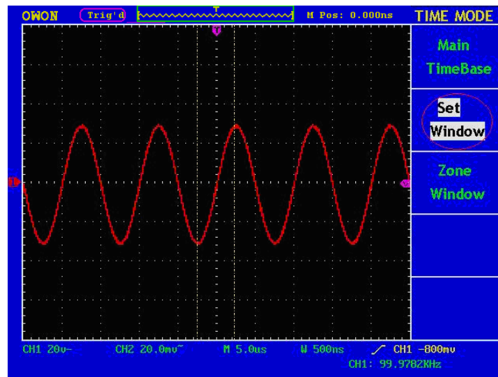
Fig. 5-16 Window Setting
