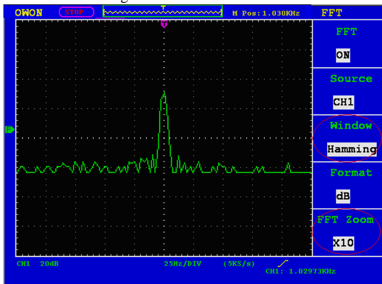
Fig.5-10 Hamming window
