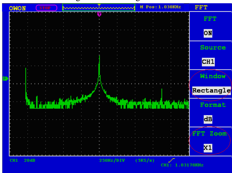
Fig.5-11. Rectangle window
