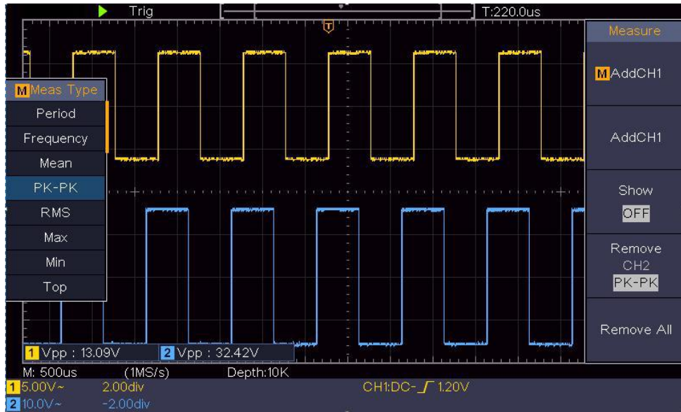
Figure 7- 2 Waveform of Gain Measurement
