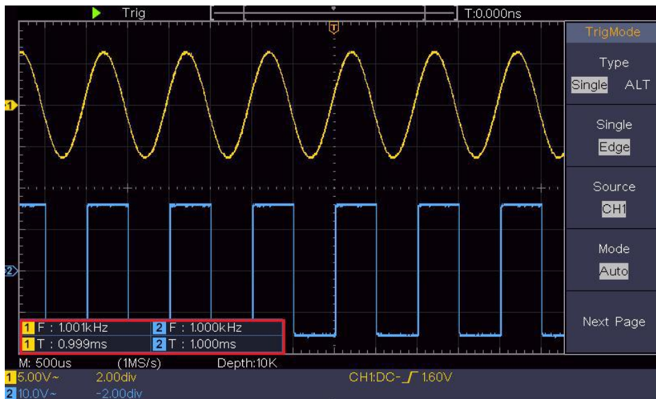
Figure 7- 1 Measure period and frequency value for a given signal
