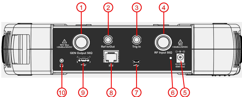
Figure 4-2 Top panel
