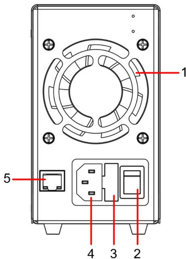
Figure 3- 3 Rear Panel Overview (With LAN model)
