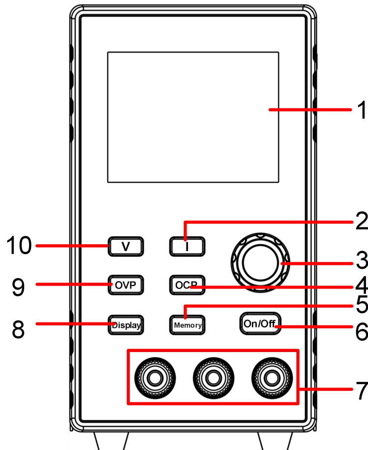
Figure 3-1 Front Panel Overview
